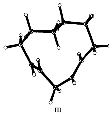
Fig. 1. Conformations I, II and III of cycloundeca-1,4-diene.
